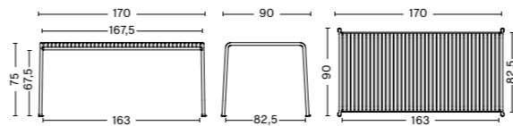
PALISSADE TABLE Length 170 cm Width 90 cm Heigth 75 cm
