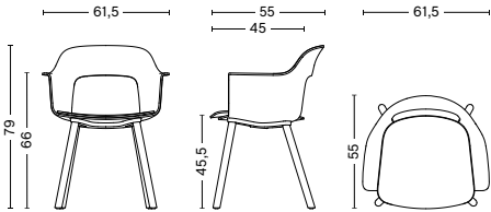
LAYOUT ARMCHAIR 221 Width 61,5 cm Depth 55 cm Height 79 cm Seat height 45,5 cm Armrest height 66 cm Weight 7,85 kg
