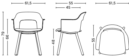
LAYOUT ARMCHAIR 223 Width 61,5 cm Depth 55 cm Height 79 cm Seat height 48 cm Armrest height 66 cm Weight 8,45 kg
