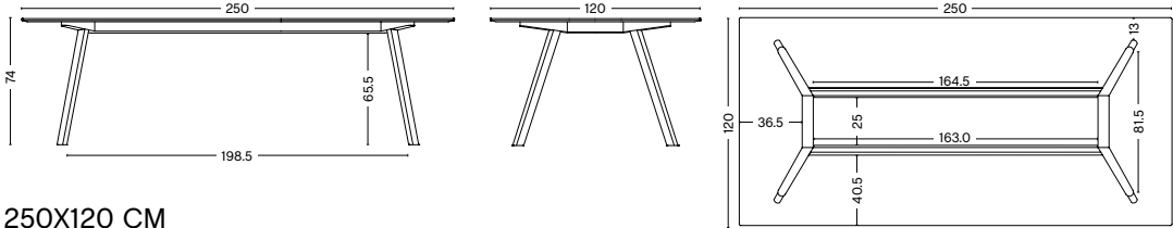
250X120 CM Width 250 cm Depth 120 cm Height 74 cm Weight 105 kg
