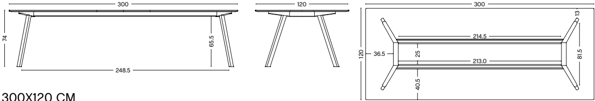
300X120 CM Width 300 cm Depth 120 cm Height 74 cm Weight 117 kg
