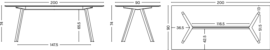
200X90 CM Width 200 cm Depth 90 cm Height 74 cm Weight 45,5 kg
